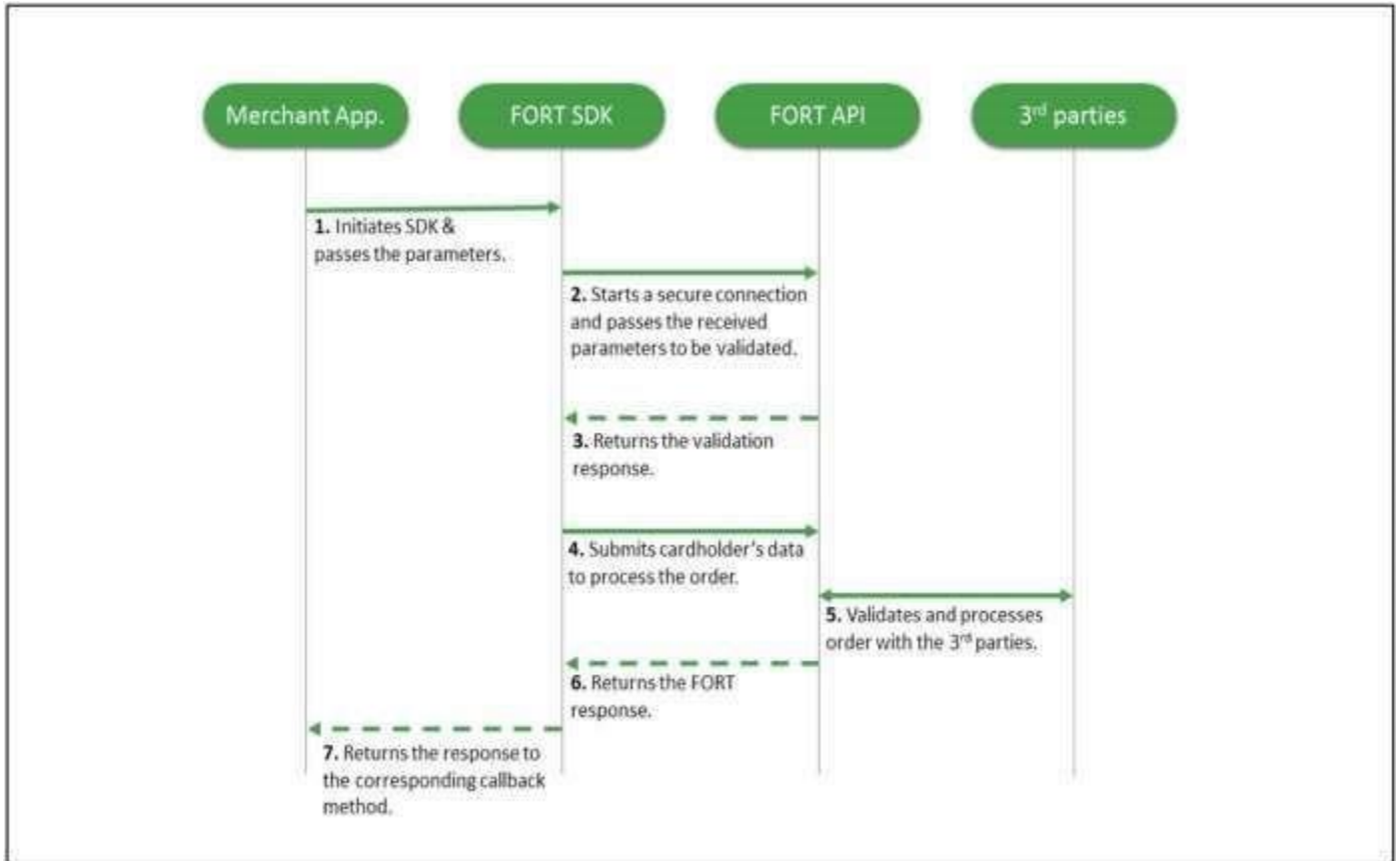
Figure 1: Payment Workflow
